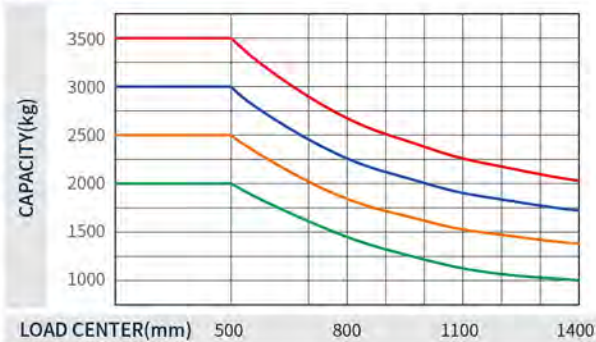
Load curve
