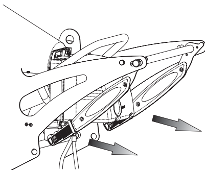
Figura 8 - Ruheposition XL9.
