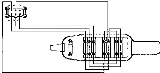
CONECTOR MACHO BOTONERA N°1
